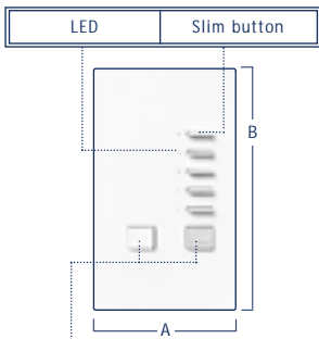
All on/All off HWI-KP5 A = 2.75" (70.0mm) B = 4.50" (114.0mm)
