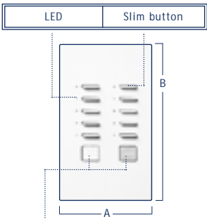
All on/All off HWI-KP10 A = 2.75" (70.0mm) B = 4.50" (114.0mm)
